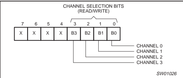
Figure 4. Control register
